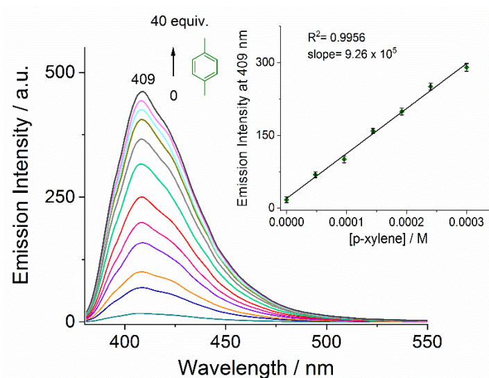
Figure 10. Changes in the emission spectra ( \lambda_{\text{ex}} = 330 nm) of acetonitrile suspension of 1 upon addition of increasing amounts of p-xylene (0–300 \mu\text{M} ). The inset shows the calibration curve with a linear fit at \lambda_{\text{em}} = 409 nm (average of triplicate experiments).
