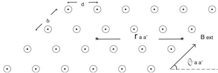
Fig. 2. Regular qubit chains define planes.
